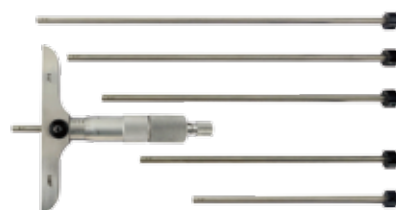
Depth Micrometer
